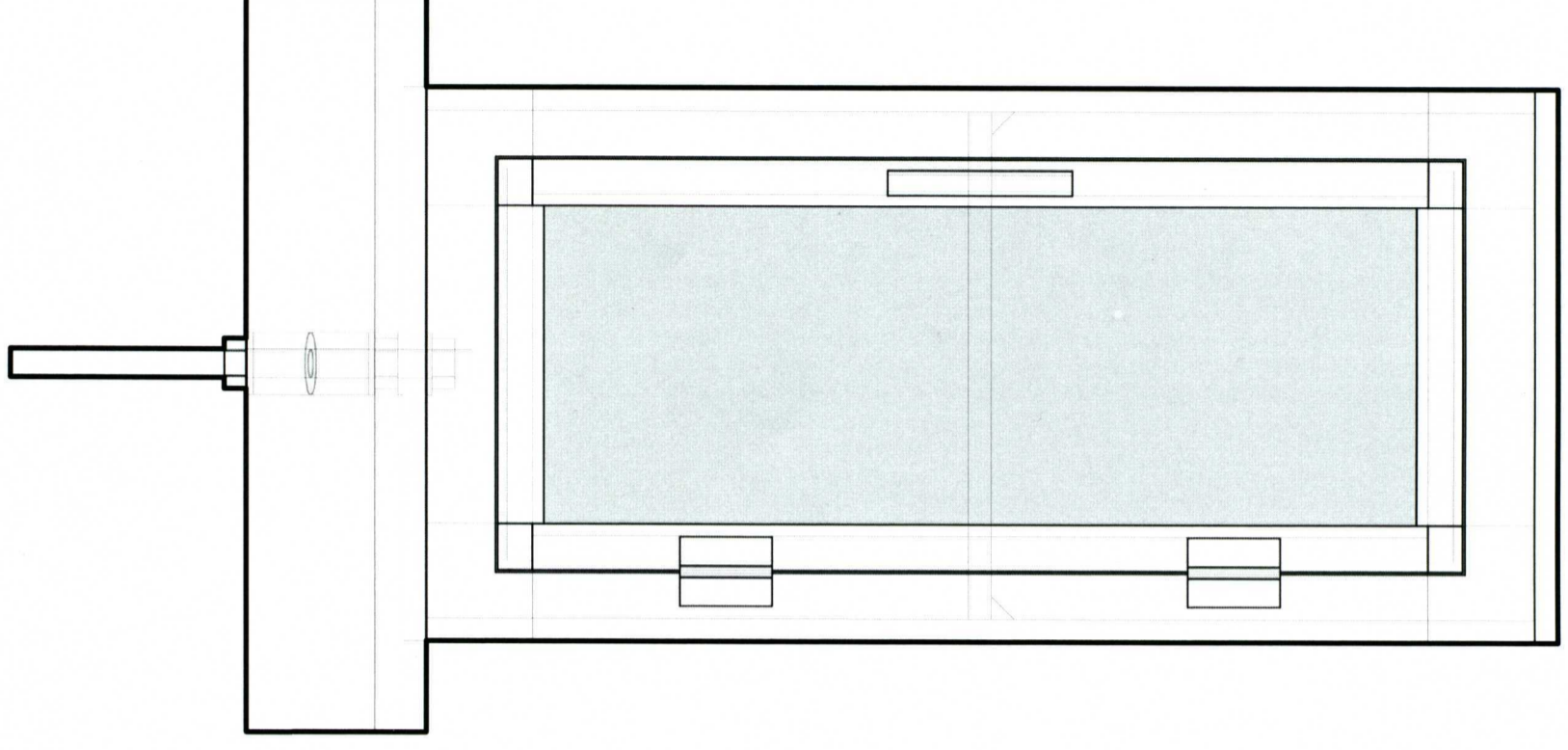
FRONT ELEVATION
